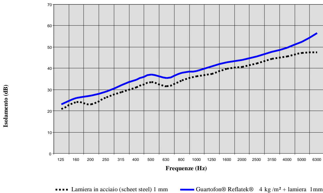
Transmission Loss + lamiera in acciaio (sheet steel)
