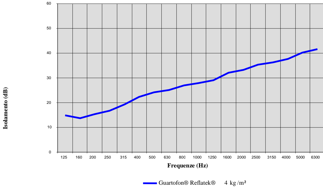
Transmission Loss (DIN 52210)
