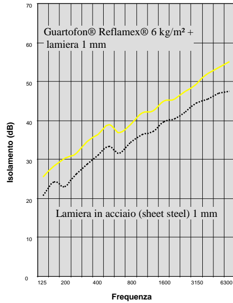
Transmission Loss + lamiera acciaio (steel sheet)
